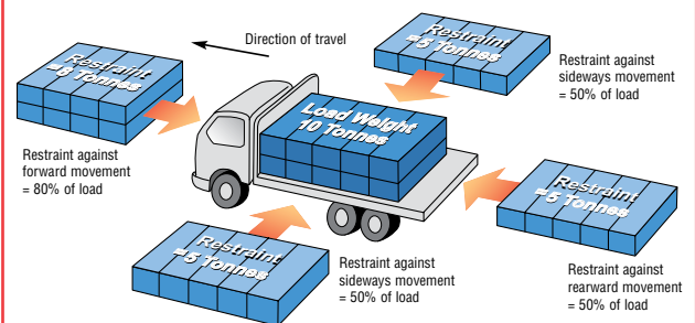
Minimum Horizontal Restraint
