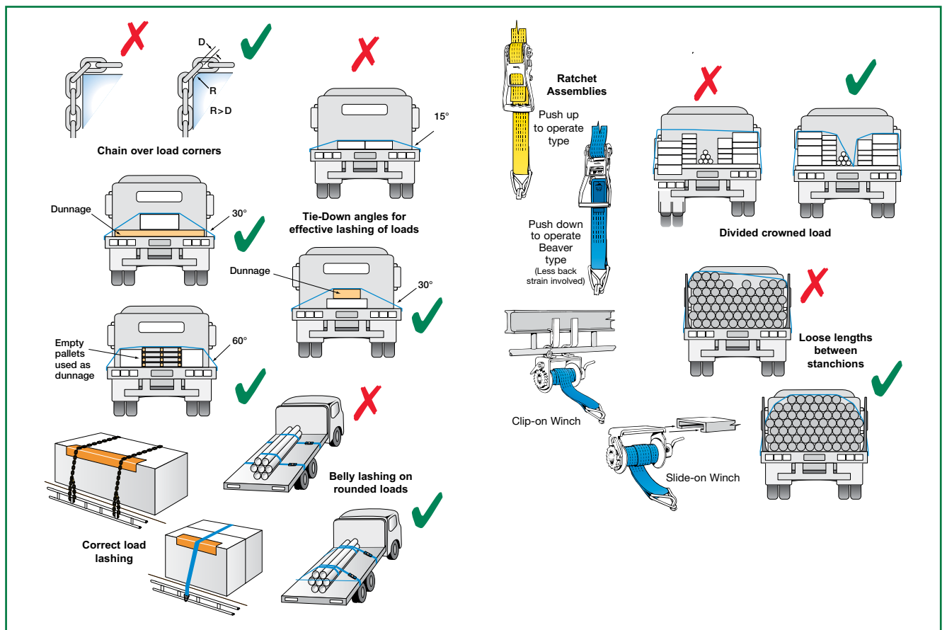
Minimum Horizontal Restraint
