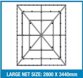
LARGE NET SIZE: 2800 X 3440mm
